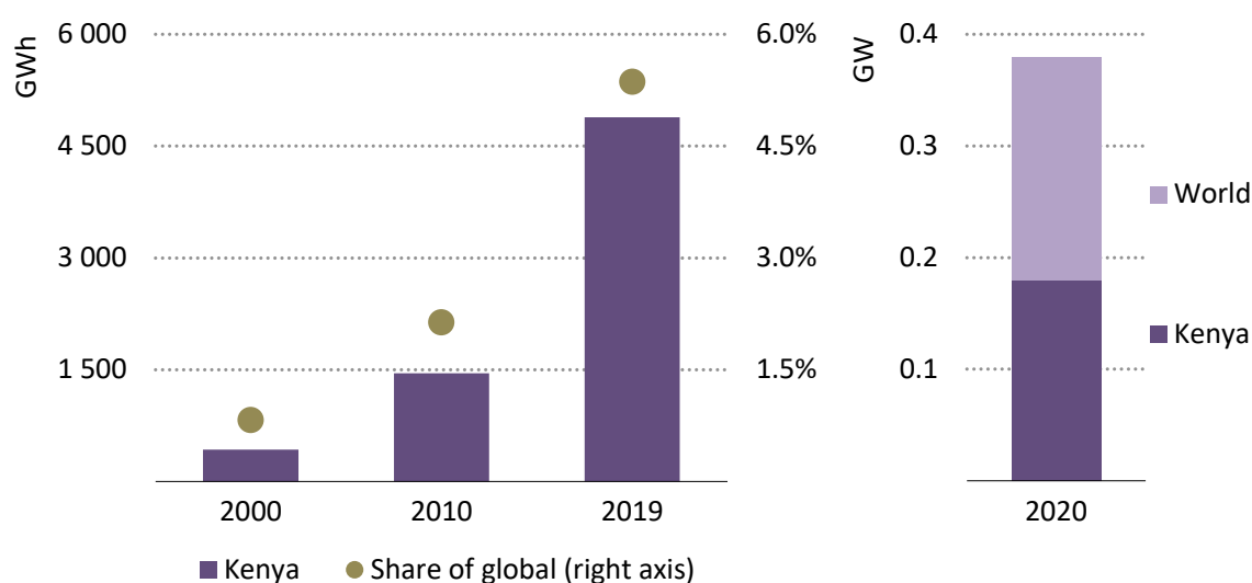
Geothermal electricity generation in Kenya and globally, 2000-2019 (left) and added capacity, 2020 (right)
